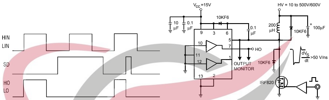
Figure 1. Input/Output Timing Diagram
